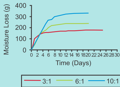
FIGURE 1 - PRE-TREATED PRATLIPERL Rate of Loss of Moulding Moisture
