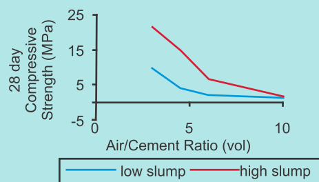
FIGURE 7 - PRE-TREATED PRATLIPERL Air/Cement Ratio (vol) vs Compressive Strength
