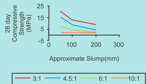
FIGURE 4 - PRE-TREATED PRATLIPERL Approximate Slump vs Compressive Strength
